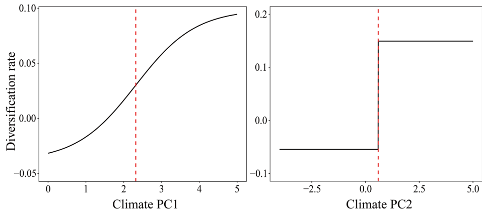
Fig. 4. Relationship between the diversification rate of the section Cyclobalanopsis and the principal components of climate variables based on QuaSSE analysis.
